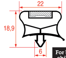
REPA IT PROFILE CODE - 3016 REPA DE PROFILE CODE - 8794
