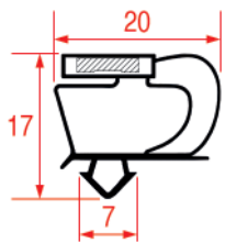
REPA IT PROFILE CODE - 1083 REPA DE PROFILE CODE - 9052
