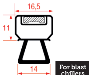
REPA IT PROFILE CODE - 8166 REPA DE PROFILE CODE - 8166
