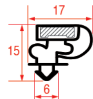
REPA IT PROFILE CODE - 1056 REPA DE PROFILE CODE - 9154
