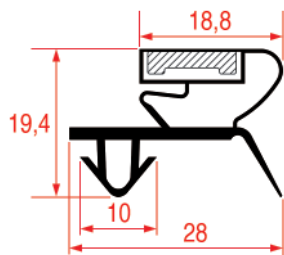
REPA IT PROFILE CODE - 1054 REPA DE PROFILE CODE - 9044
