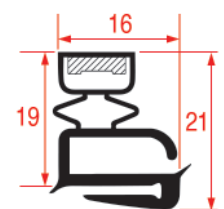
REPA IT PROFILE CODE - 2017 REPA DE PROFILE CODE - 9100
