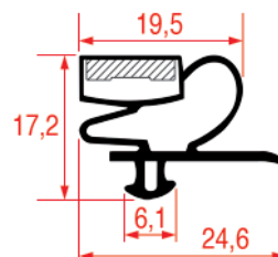
REPA IT PROFILE CODE - 1009 REPA DE PROFILE CODE - 9012
