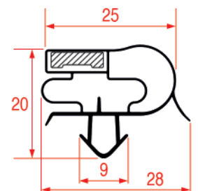
REPA IT PROFILE CODE - 1078 REPA DE PROFILE CODE - 9167
