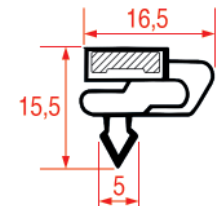
REPA IT PROFILE CODE - 1092 REPA DE PROFILE CODE - 9156
