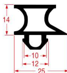
REPA DE PROFILE CODE - 9172
