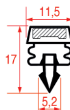
REPA IT PROFILE CODE - 1081 REPA DE PROFILE CODE - 9314
