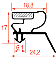
REPA IT PROFILE CODE - 1074 REPA DE PROFILE CODE - 9400
