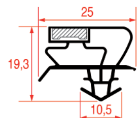
REPA IT PROFILE CODE - 1035 REPA DE PROFILE CODE - 9055
