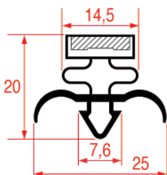
REPA IT PROFILE CODE - 1023 REPA DE PROFILE CODE - 9171
