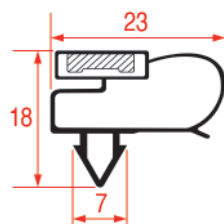
REPA IT PROFILE CODE - 1062 REPA DE PROFILE CODE - 9051
