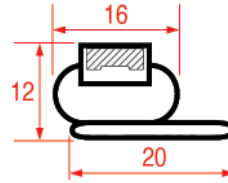
REPA IT PROFILE CODE - 2021 REPA DE PROFILE CODE - 9968
