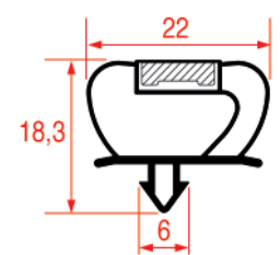
REPA IT PROFILE CODE - 1010 REPA DE PROFILE CODE - 9237
