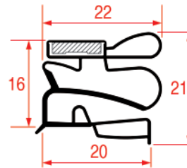
REPA IT PROFILE CODE - 2025 REPA DE PROFILE CODE - 9035
