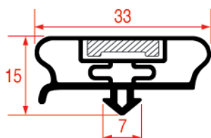
REPA IT PROFILE CODE - 1033 REPA DE PROFILE CODE - 9800
