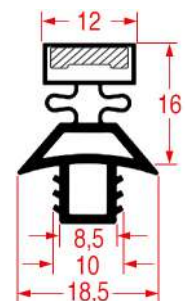
REPA DE PROFILE CODE - 9320
