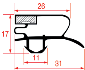
REPA IT PROFILE CODE - 1044 REPA DE PROFILE CODE - 9018
