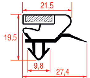
REPA IT PROFILE CODE - 1073 REPA DE PROFILE CODE - 9398
