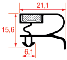
REPA IT PROFILE CODE - 1014 REPA DE PROFILE CODE - 9753
