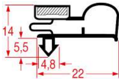
REPA DE PROFILE CODE - 9763
