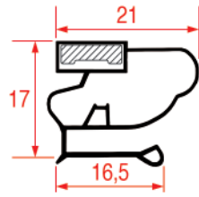
REPA IT PROFILE CODE - 2019 REPA DE PROFILE CODE - 9135
