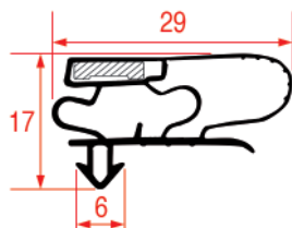
REPA IT PROFILE CODE - 1071 REPA DE PROFILE CODE - 9014
