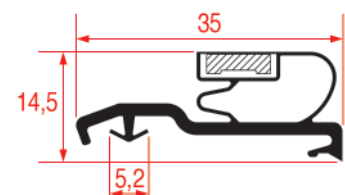
REPA IT PROFILE CODE - 1066 REPA DE PROFILE CODE - 9724
