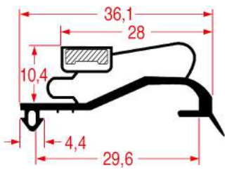
REPA DE PROFILE CODE - 9725
