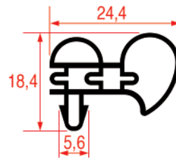
REPA IT PROFILE CODE - 1027 REPA DE PROFILE CODE - 9431
