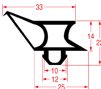
REPA DE PROFILE CODE - 9173
