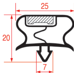
REPA IT PROFILE CODE - 1058 REPA DE PROFILE CODE - 9197
