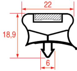
REPA IT PROFILE CODE - 1016 REPA DE PROFILE CODE - 9794
