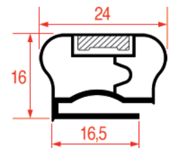
REPA IT PROFILE CODE - 2009 REPA DE PROFILE CODE - 9200
