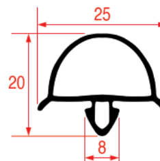
REPA IT PROFILE CODE - 1047 REPA DE PROFILE CODE - 9729
