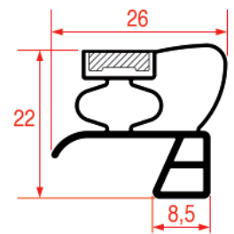
REPA IT PROFILE CODE - 1002 REPA DE PROFILE CODE - 9783
