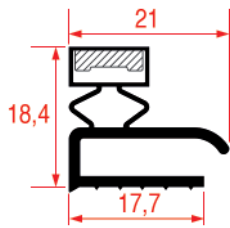
REPA IT PROFILE CODE - 2002 REPA DE PROFILE CODE - 9106
