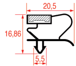
REPA IT PROFILE CODE - 1038 REPA DE PROFILE CODE - 9053
