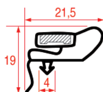
REPA IT PROFILE CODE - 1050 REPA DE PROFILE CODE - 9952
