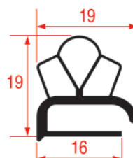
REPA IT PROFILE CODE - 2016 REPA DE PROFILE CODE - 9191
