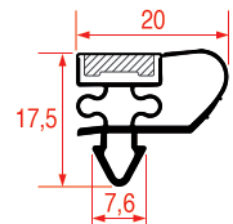
REPA IT PROFILE CODE - 1022 REPA DE PROFILE CODE - 9153
