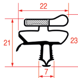
REPA IT PROFILE CODE - 1088 REPA DE PROFILE CODE - 9023
