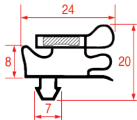
REPA IT PROFILE CODE - 1084 REPA DE PROFILE CODE - 9042
