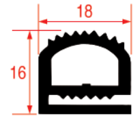
REPA IT PROFILE CODE - 2022 REPA DE PROFILE CODE - 9170
