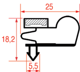
REPA IT PROFILE CODE - 1007 REPA DE PROFILE CODE - 9010
