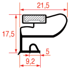
REPA IT PROFILE CODE - 2001 REPA DE PROFILE CODE - 9663
