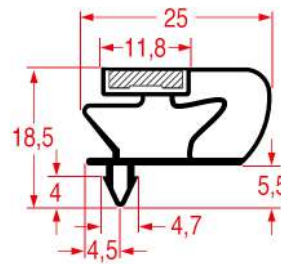
REPA DE PROFILE CODE - 9799
