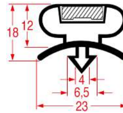
REPA DE PROFILE CODE - 9199
