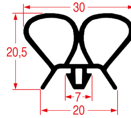
REPA DE PROFILE CODE - 9938
