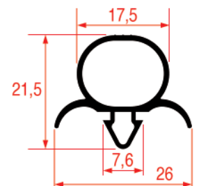
REPA IT PROFILE CODE - 1032 REPA DE PROFILE CODE - 9192
