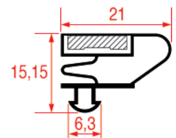
REPA IT PROFILE CODE - 1006 REPA DE PROFILE CODE - 9703
