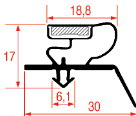
REPA IT PROFILE CODE - 1075 REPA DE PROFILE CODE - 9401
