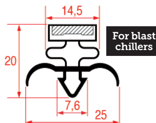
REPA IT PROFILE CODE - 8171 REPA DE PROFILE CODE - 8171
