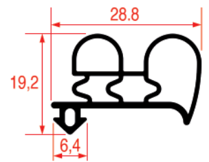
REPA IT PROFILE CODE - 1028 REPA DE PROFILE CODE - 9430
