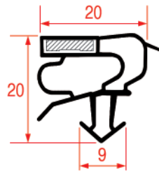
REPA IT PROFILE CODE - 1085 REPA DE PROFILE CODE - 9152
