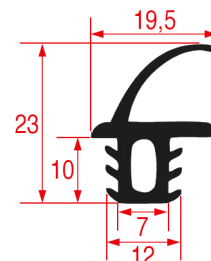
REPA DE PROFILE CODE - 9299
