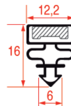
REPA IT PROFILE CODE - 1059 REPA DE PROFILE CODE - 9313
