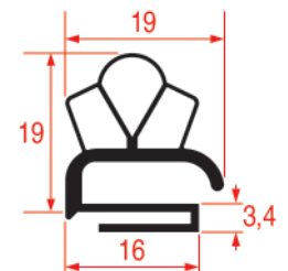
REPA IT PROFILE CODE - 2013 REPA DE PROFILE CODE - 9138
