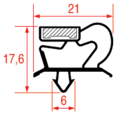
REPA IT PROFILE CODE - 1001 REPA DE PROFILE CODE - 9048
