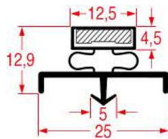
REPA DE PROFILE CODE - 9316
