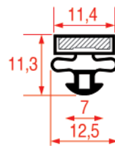
REPA IT PROFILE CODE - 1091 REPA DE PROFILE CODE - 9032
