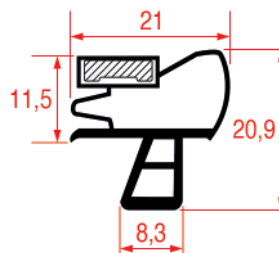
REPA IT PROFILE CODE - 1076 REPA DE PROFILE CODE - 9956
