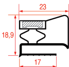
REPA IT PROFILE CODE - 2014 REPA DE PROFILE CODE - 9953
