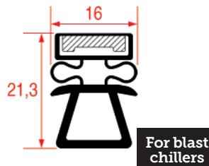
REPA IT PROFILE CODE - 8162 REPA DE PROFILE CODE - 8162
