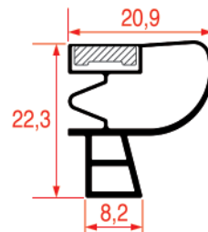
REPA IT PROFILE CODE - 1055 REPA DE PROFILE CODE - 9950
