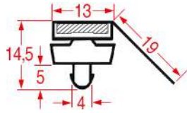
REPA DE PROFILE CODE - 9385
