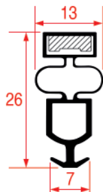
REPA IT PROFILE CODE - 1045 REPA DE PROFILE CODE - 9327
