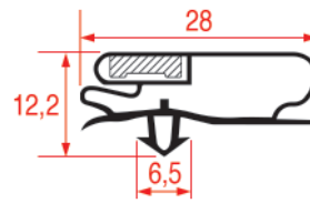
REPA IT PROFILE CODE - 1068 REPA DE PROFILE CODE - 9500
