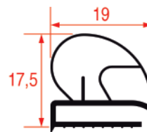
REPA IT PROFILE CODE - 2012 REPA DE PROFILE CODE - 9710
