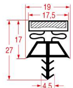
REPA DE PROFILE CODE - 9321
