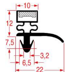
REPA DE PROFILE CODE - 9040
