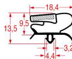
REPA DE PROFILE CODE - 9056
